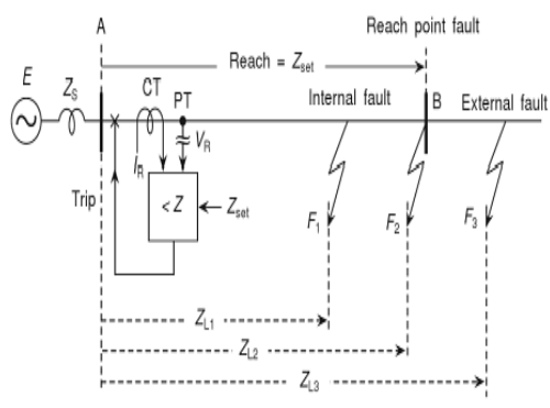
Distance Protection
