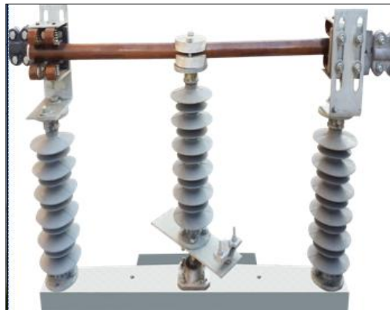
Isolator
